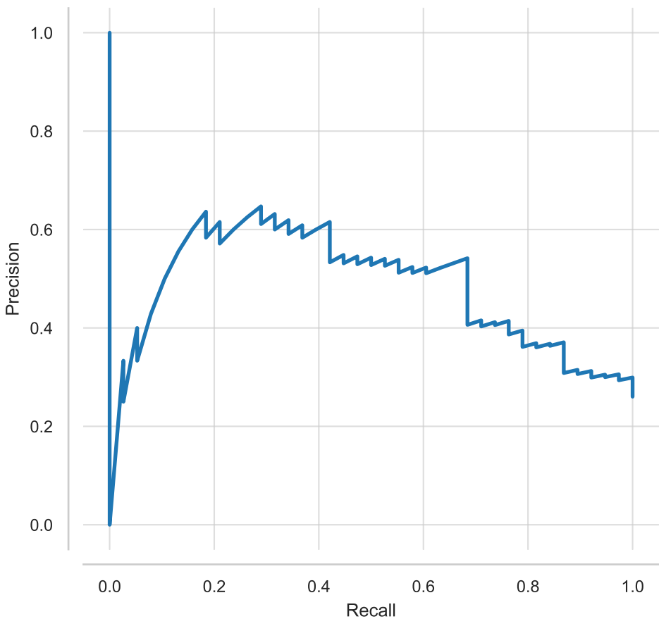
Precision-Recall Curve - RF
